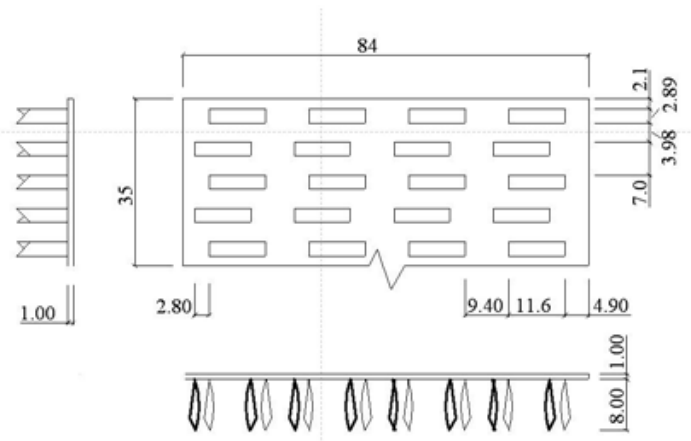
Schema conector tip GNA20:
